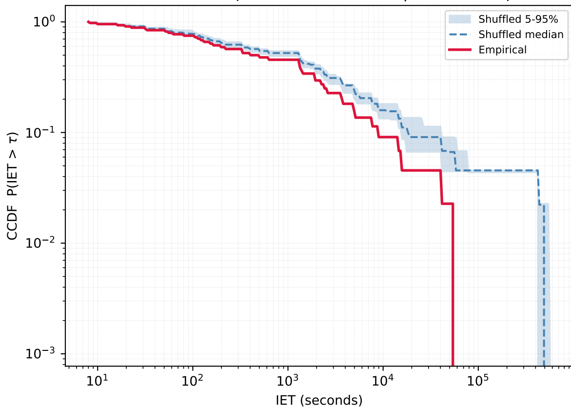
User 709835653 - Empirical vs Reshuffled | KS=0.102 p=0.010
